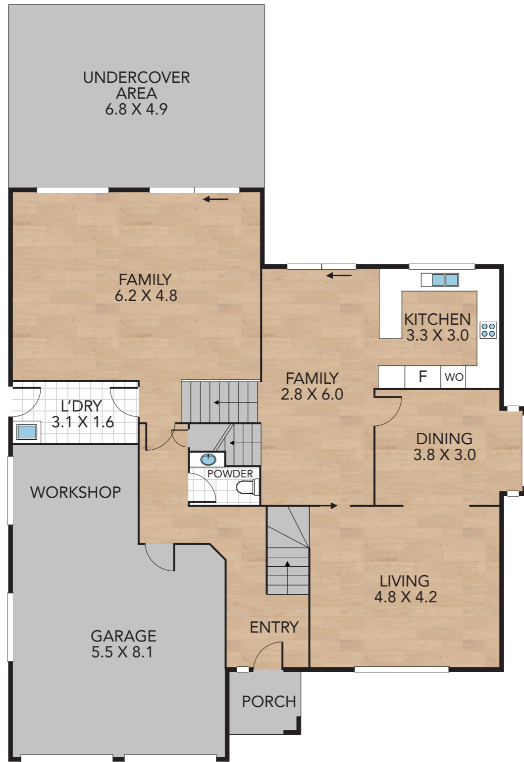
GROUND FLOOR
